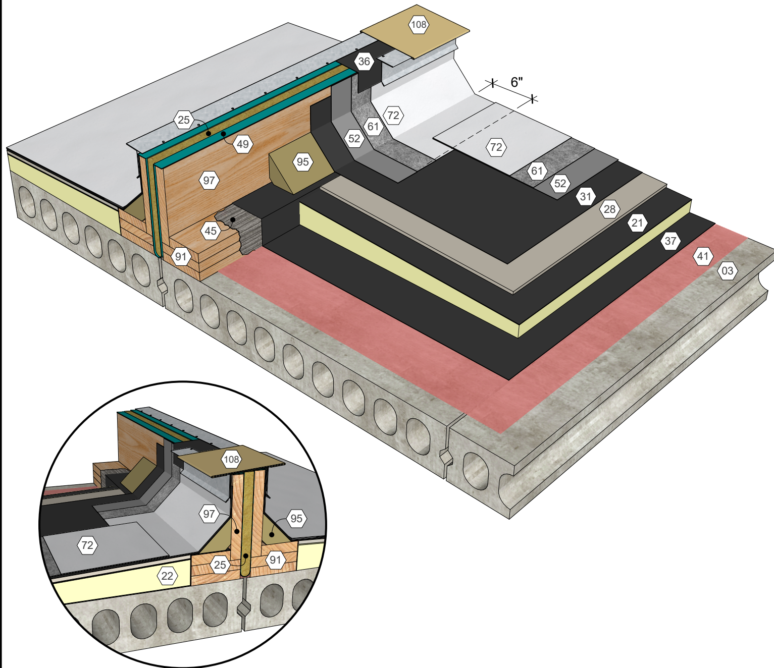
AlphaGuard® BIO Plus Expansion Joint, Temp. Roof, Precast Concrete Deck Detail 33083
