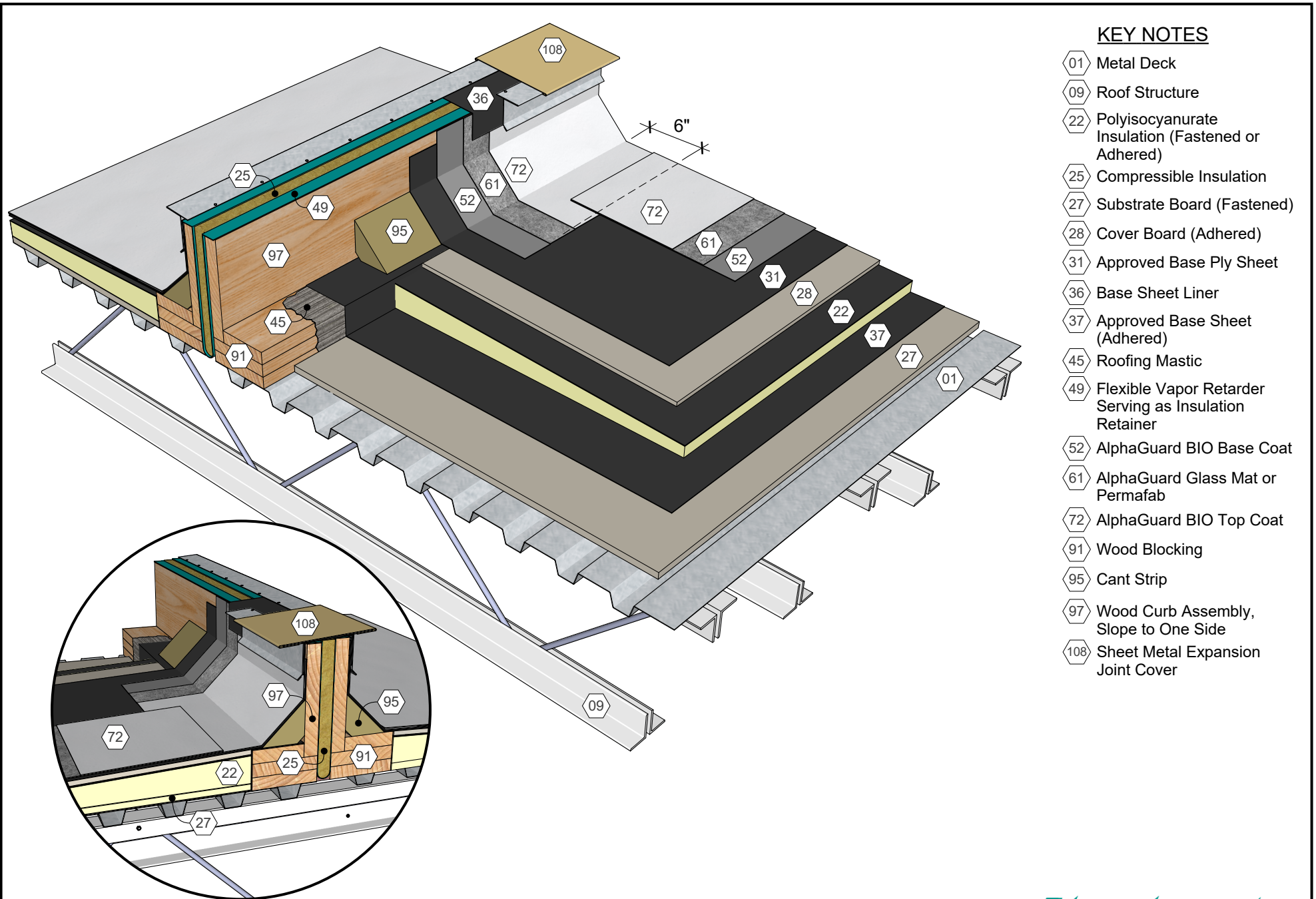
AlphaGuard® BIO Plus Expansion Joint, Temp. Roof, Metal Deck Detail 33081
