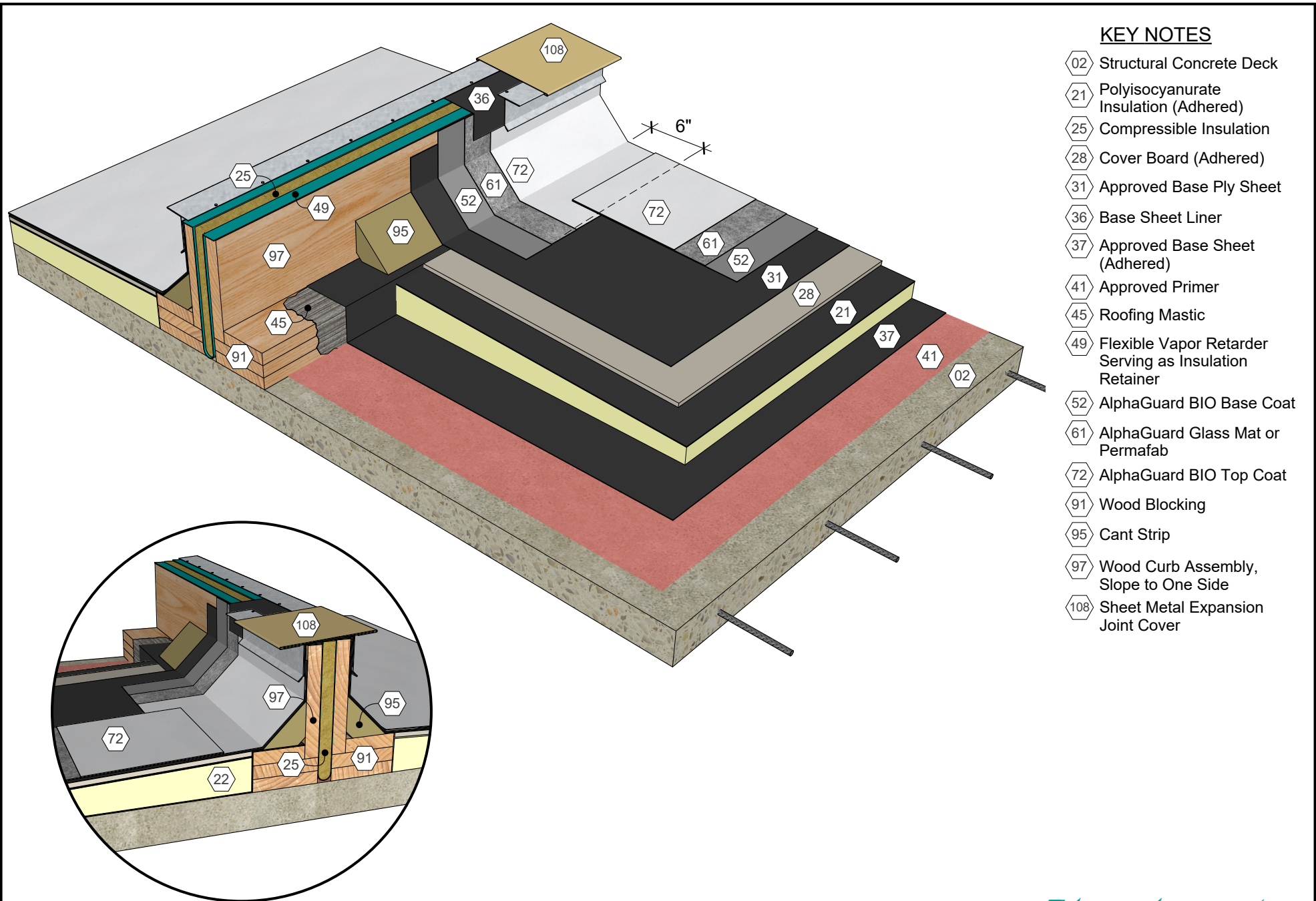
AlphaGuard® BIO Plus Expansion Joint, Temp. Roof, Structural Concrete Deck Detail 33082
