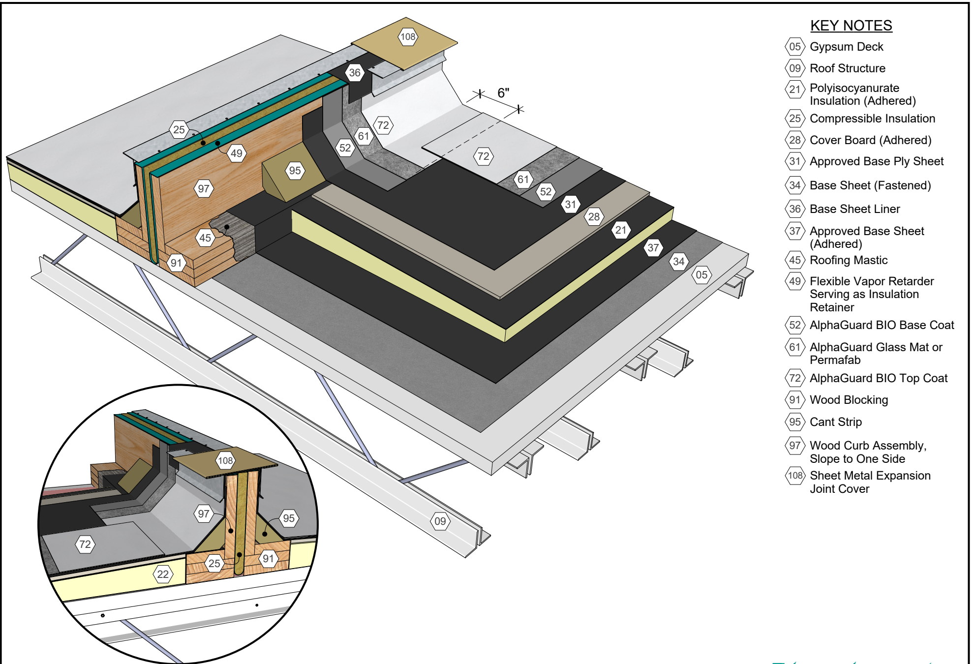
AlphaGuard® BIO Plus Expansion Joint, Temp. Roof, Gypsum Deck Detail 33085
